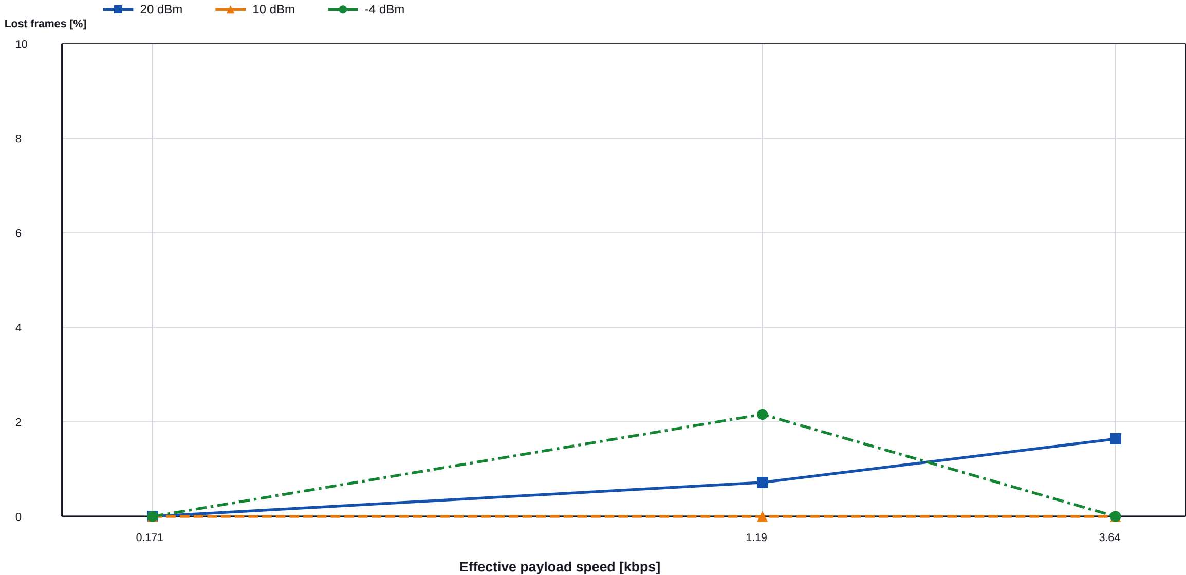
Ai-Thinker RA-02 (SX1278) + 2Cap: loss versus effective payload speed
