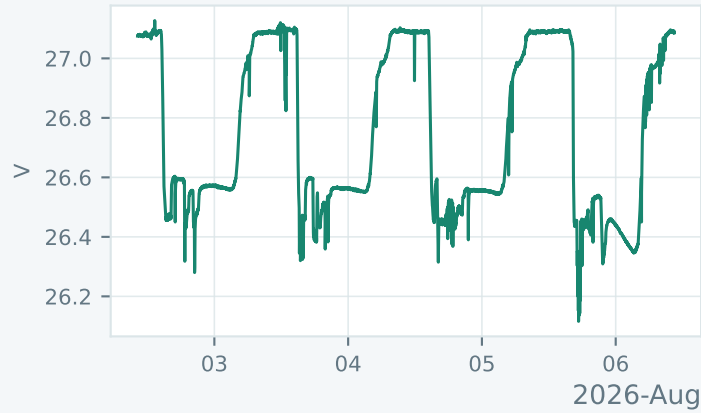
Daly BMS — Pack voltage
