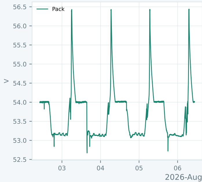
Pack voltage
