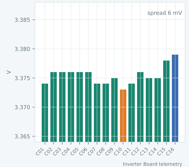
Latest individual cell voltages
