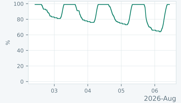
Daly BMS — State of charge
