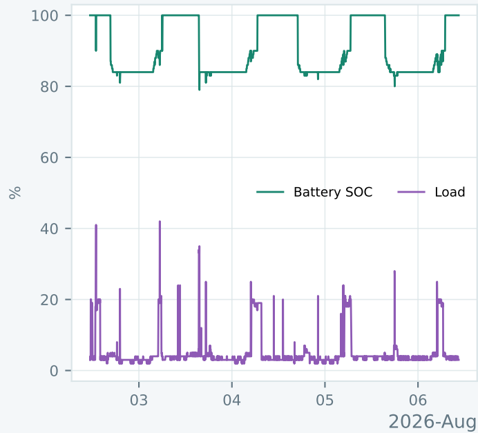
State of charge and load
