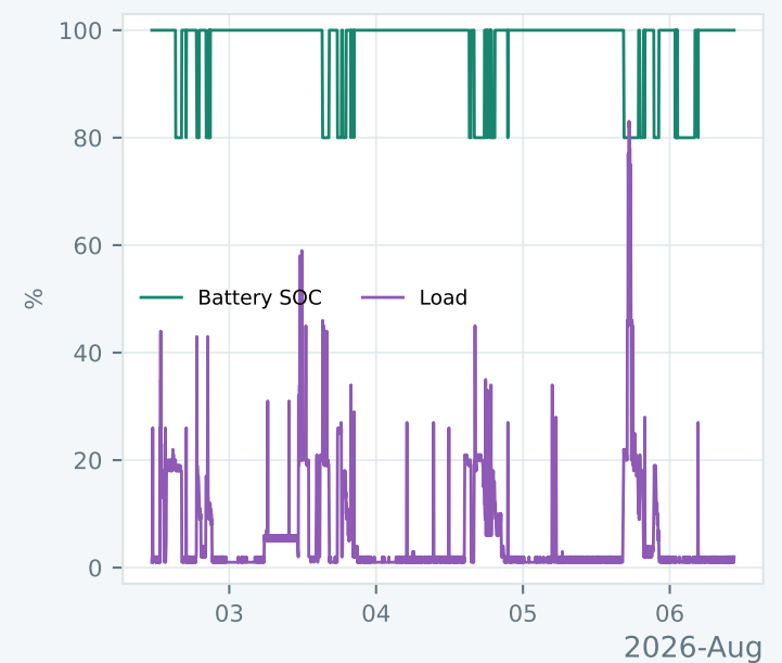
EASUN — SOC and load
