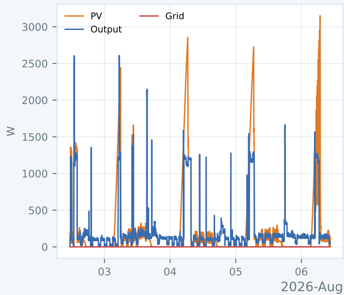
Anenji — Power
