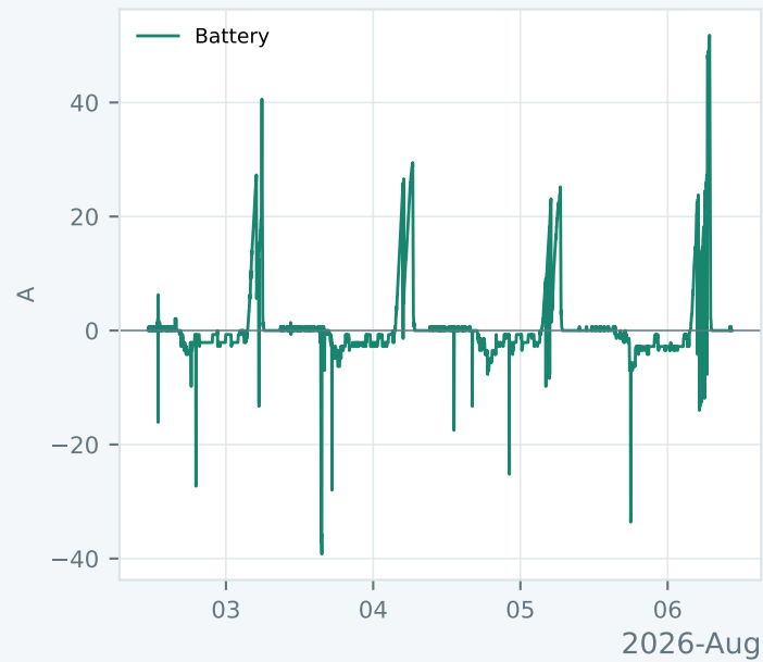
Anenji — Battery current
