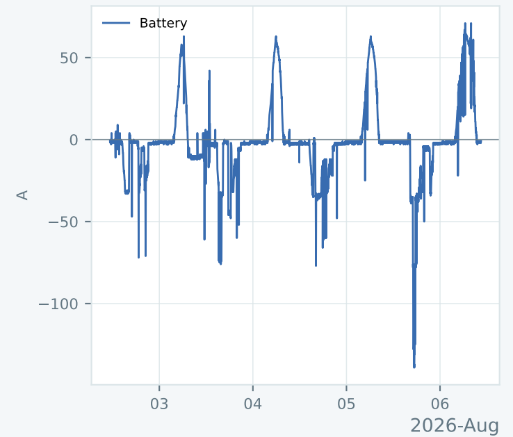
Battery current
