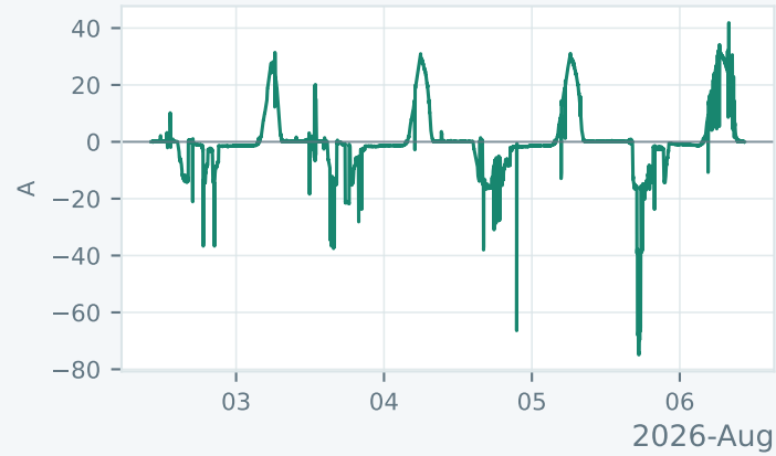
Daly BMS — Battery current
