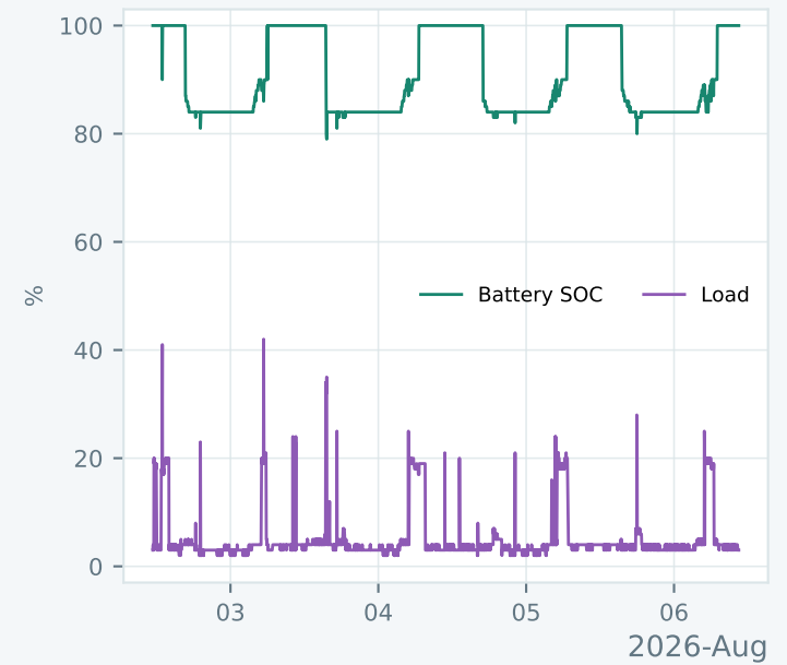
Anenji — SOC and load
