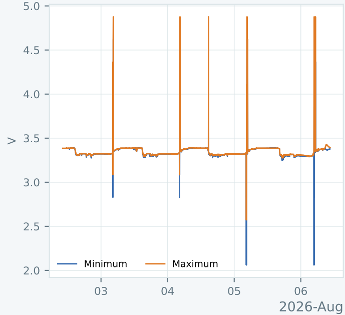
Cell voltage envelope
