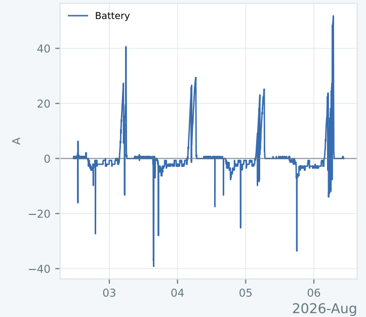
Battery current
