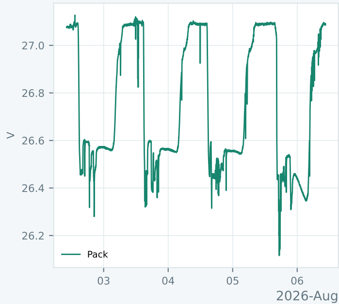
Pack voltage
