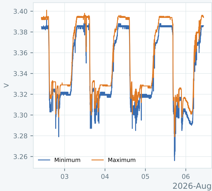
Cell voltage envelope
