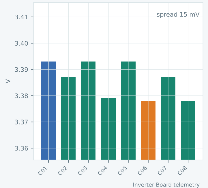
Latest individual cell voltages
