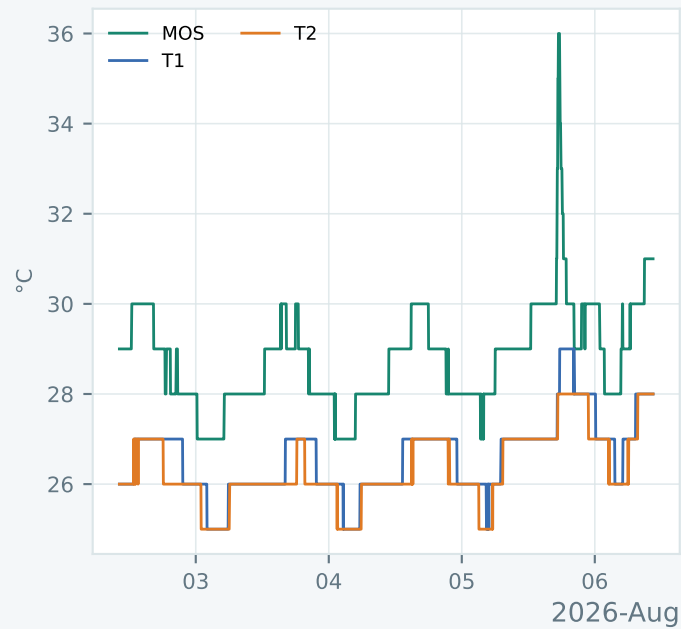
Temperatures
