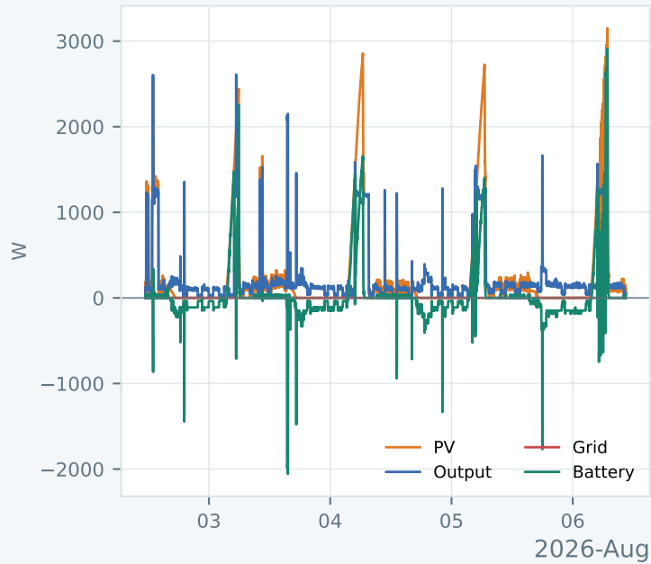
Power flow
