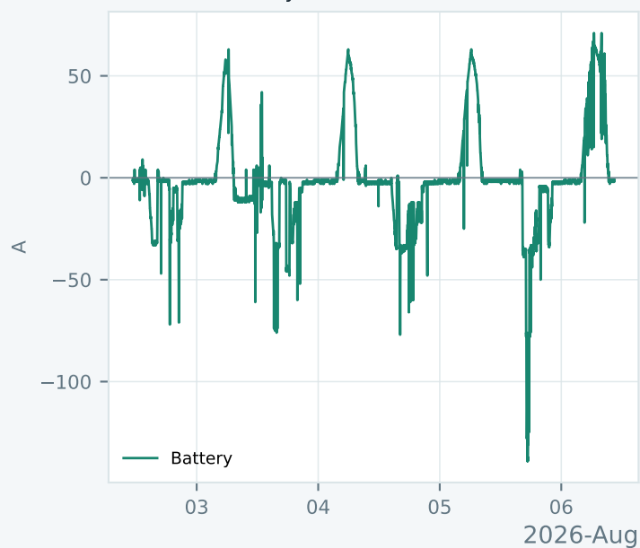
EASUN — Battery current
