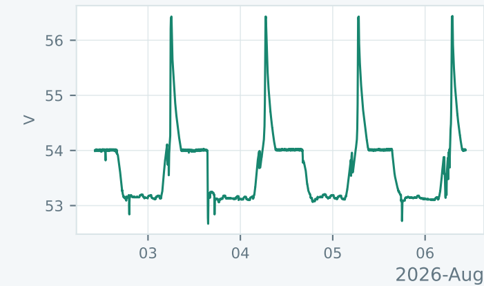
Seplos BMS — Pack voltage
