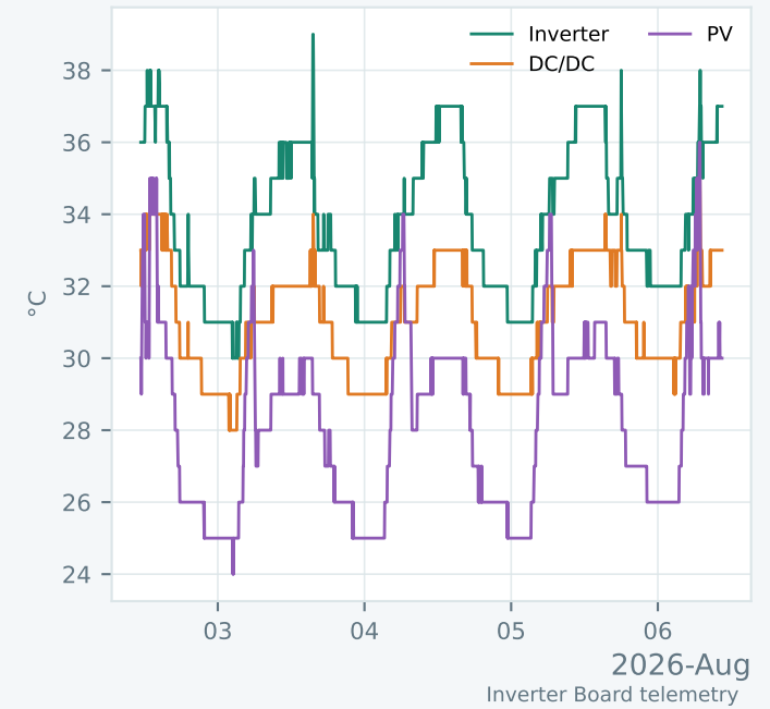
Temperatures
