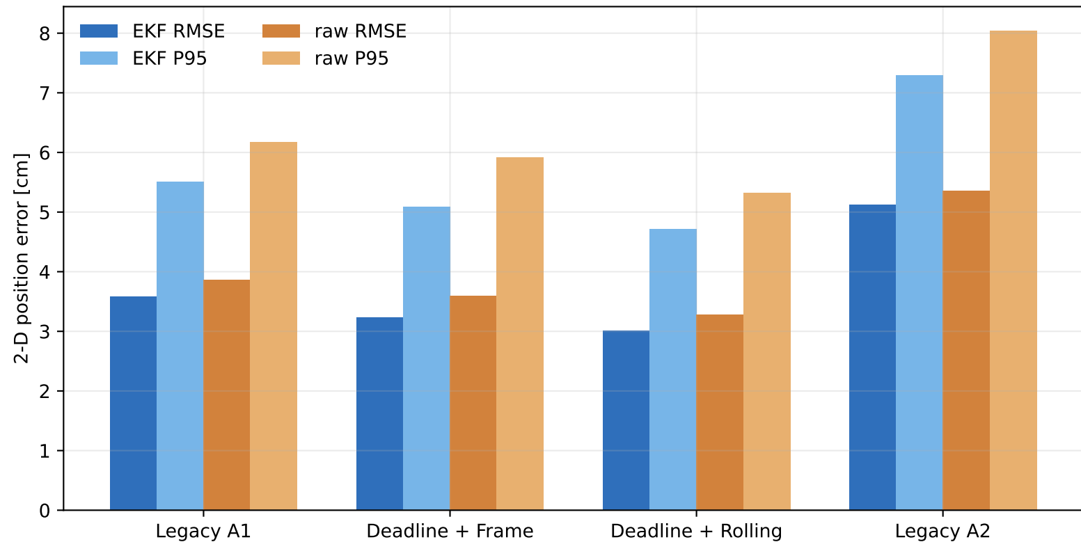
Accuracy check against the surveyed centre
