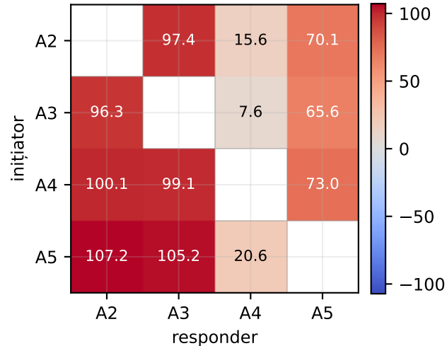
Necorectat: bias [cm]
