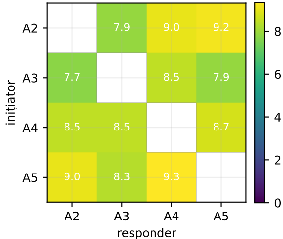
Corectat: \sigma robust (MAD) [cm]
