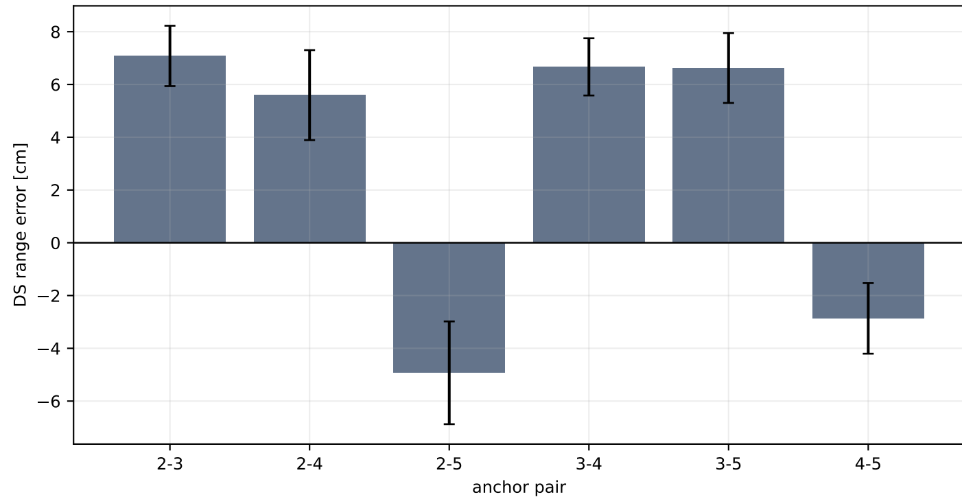
Anchor-pair DS-TWR bias (mean \pm 1\sigma )
