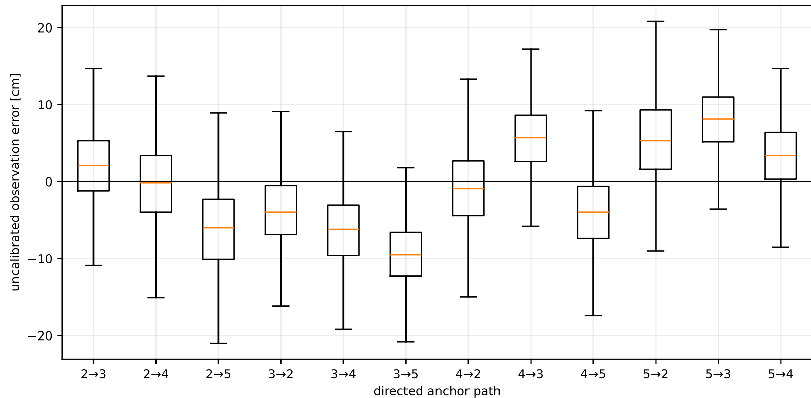
Directed observation bias before calibration
