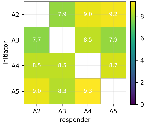
Corrected: robust \sigma (MAD) [cm]
