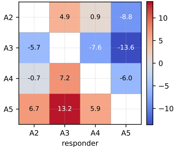
Corrected: bias [cm]
