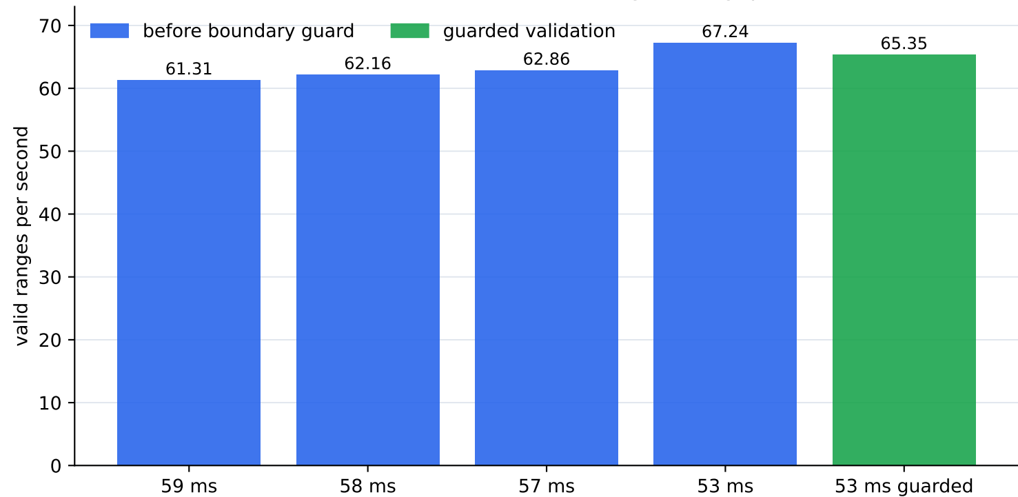
Delivered Native DS-TWR range throughput
