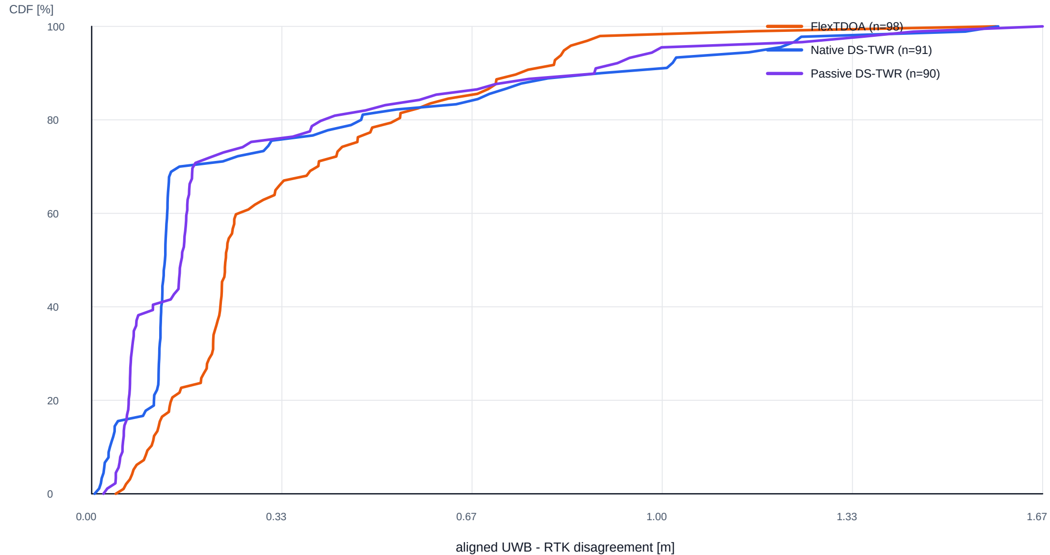
Dynamic paired error CDF (RTK is not surveyed truth)
