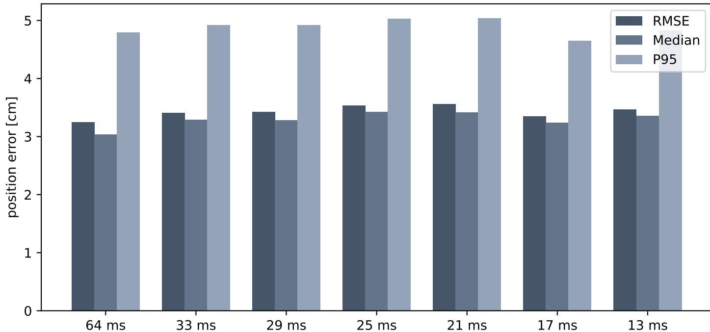
Accuracy versus DS-TWR frame period
