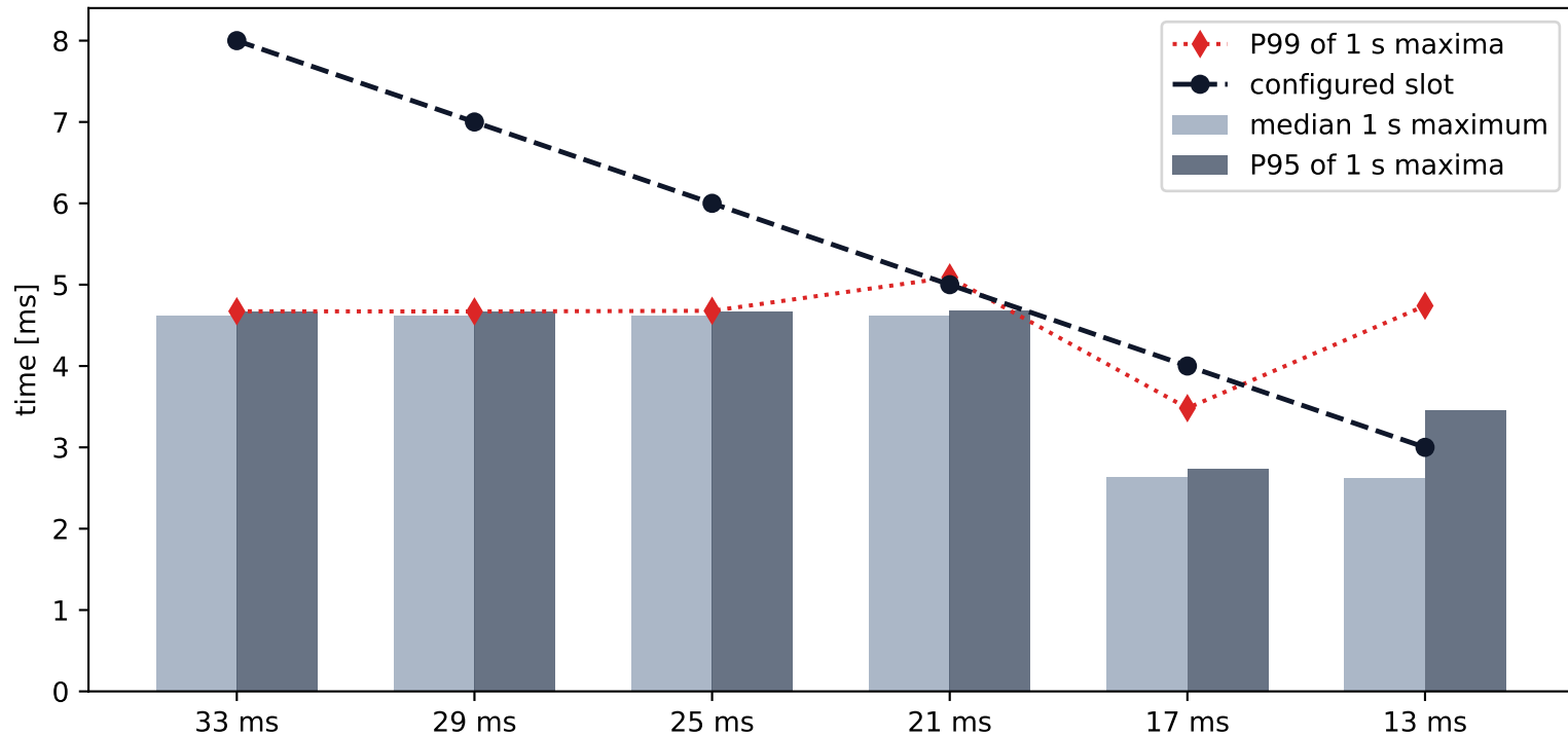
Observed exchange envelope versus slot budget
