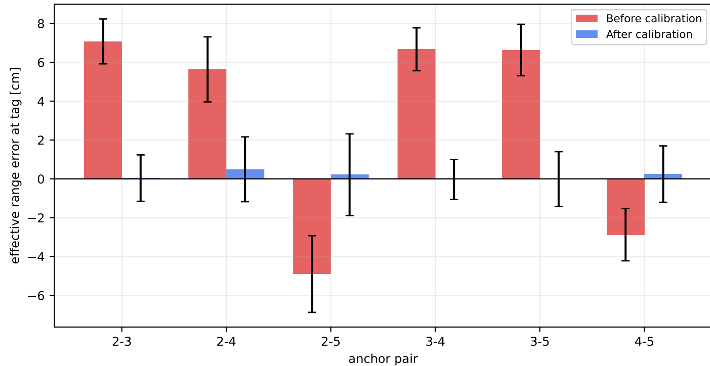
Effective anchor range: before vs after (mean \pm 1\sigma )
