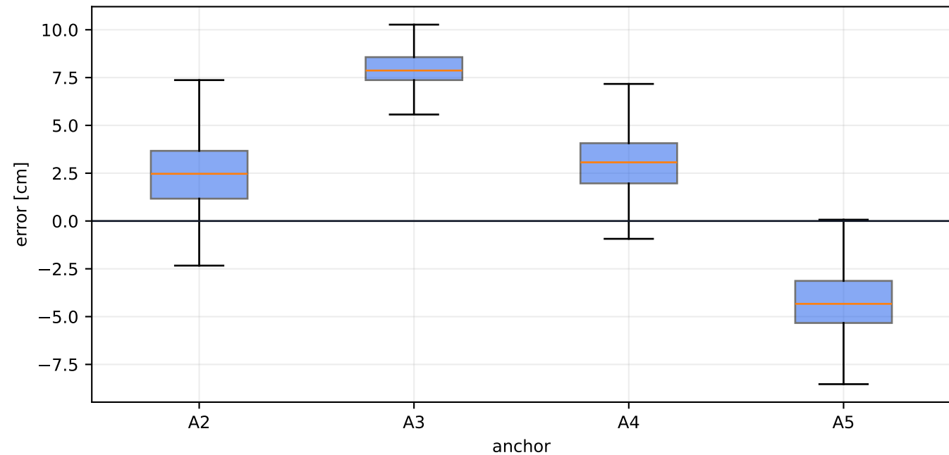
DS-TWR: range error relative to 2.12132 m
