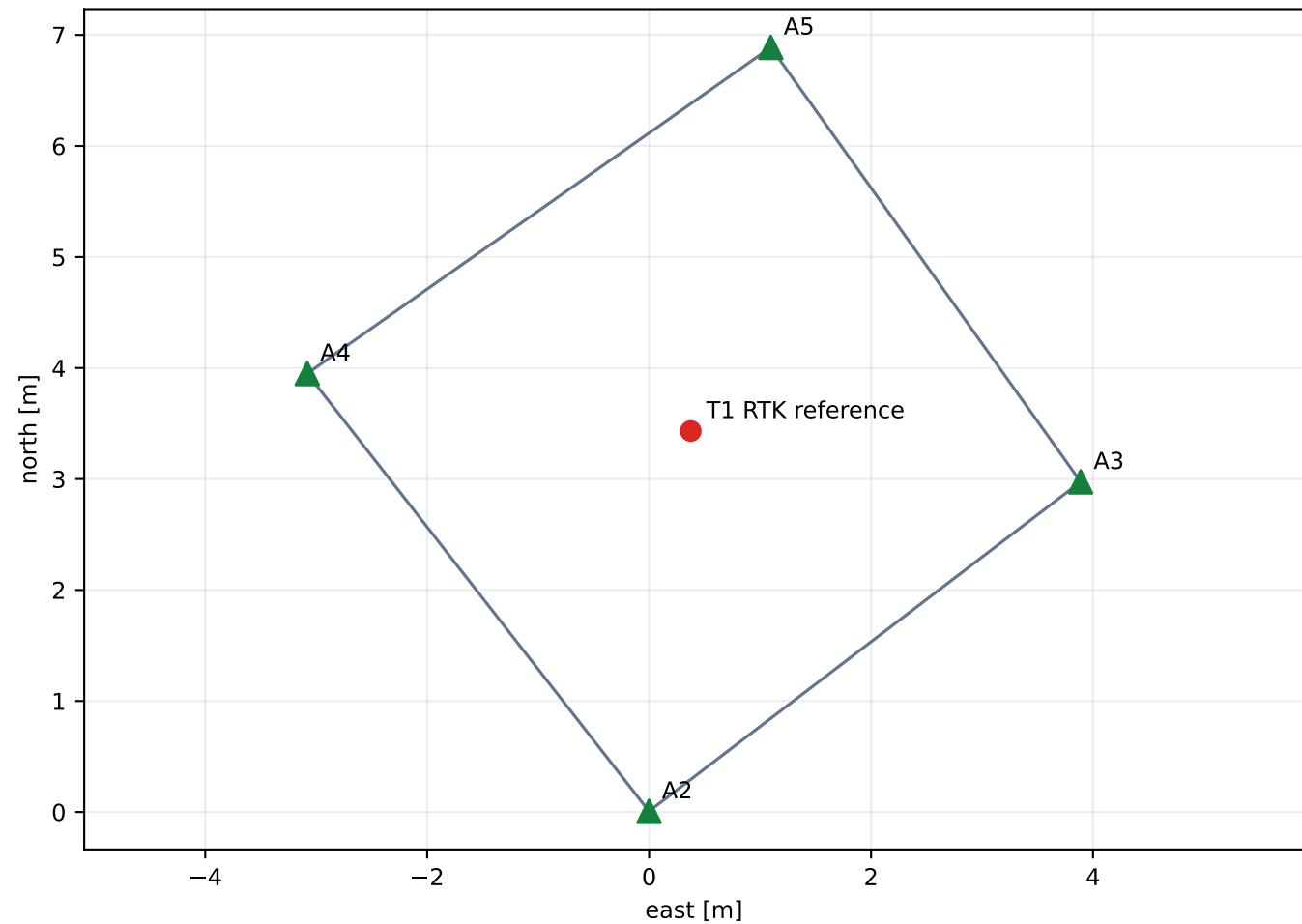
RTK-derived common analysis geometry
