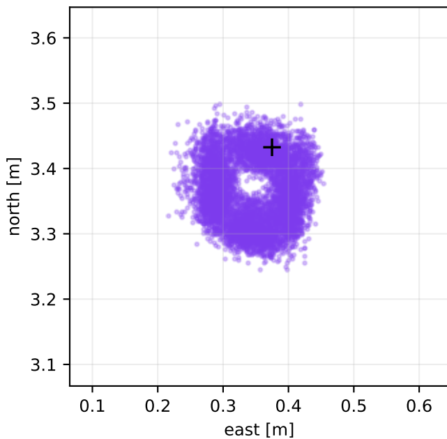
Passive DS-TWR (n=7,838)
