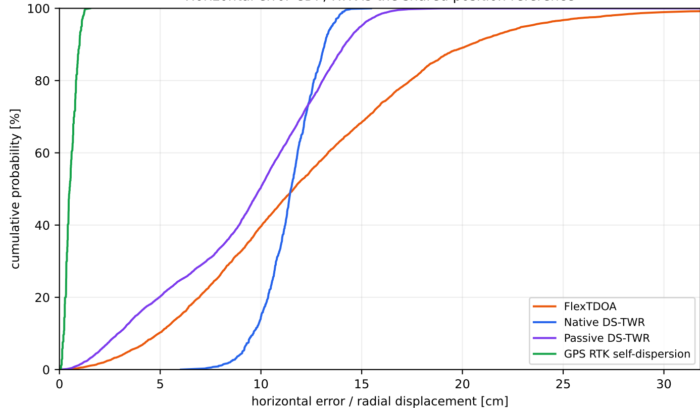
Horizontal error CDF; RTK is the shared position reference
