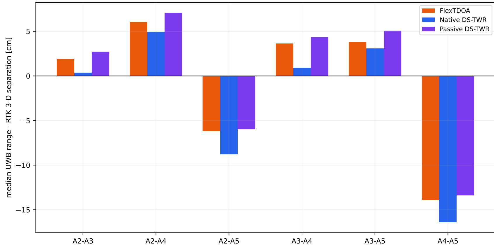
Anchor-to-anchor range bias against RTK geometry
