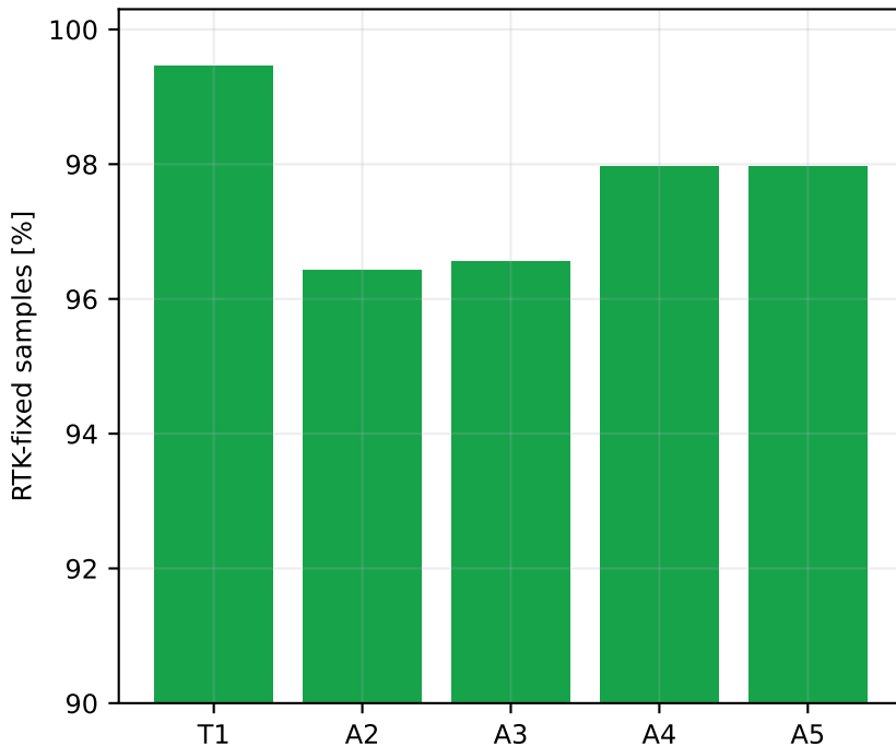
RTK availability
