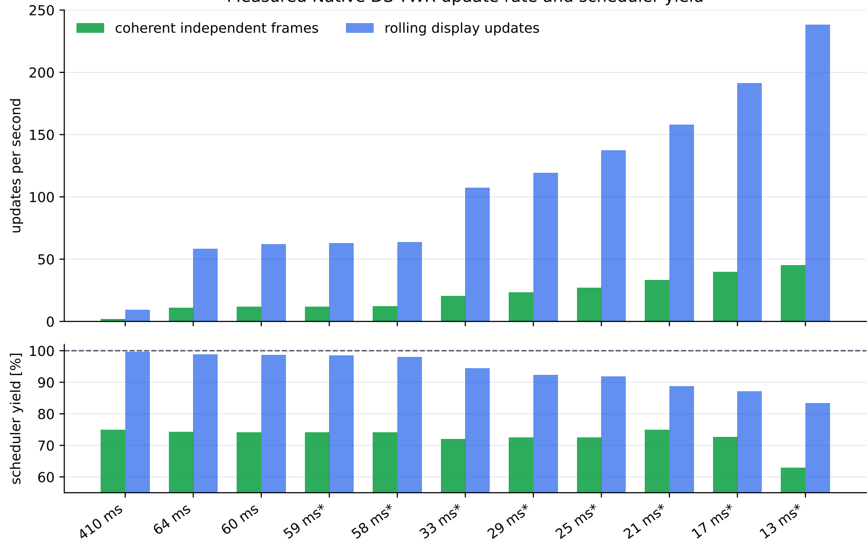
Measured Native DS-TWR update rate and scheduler yield
