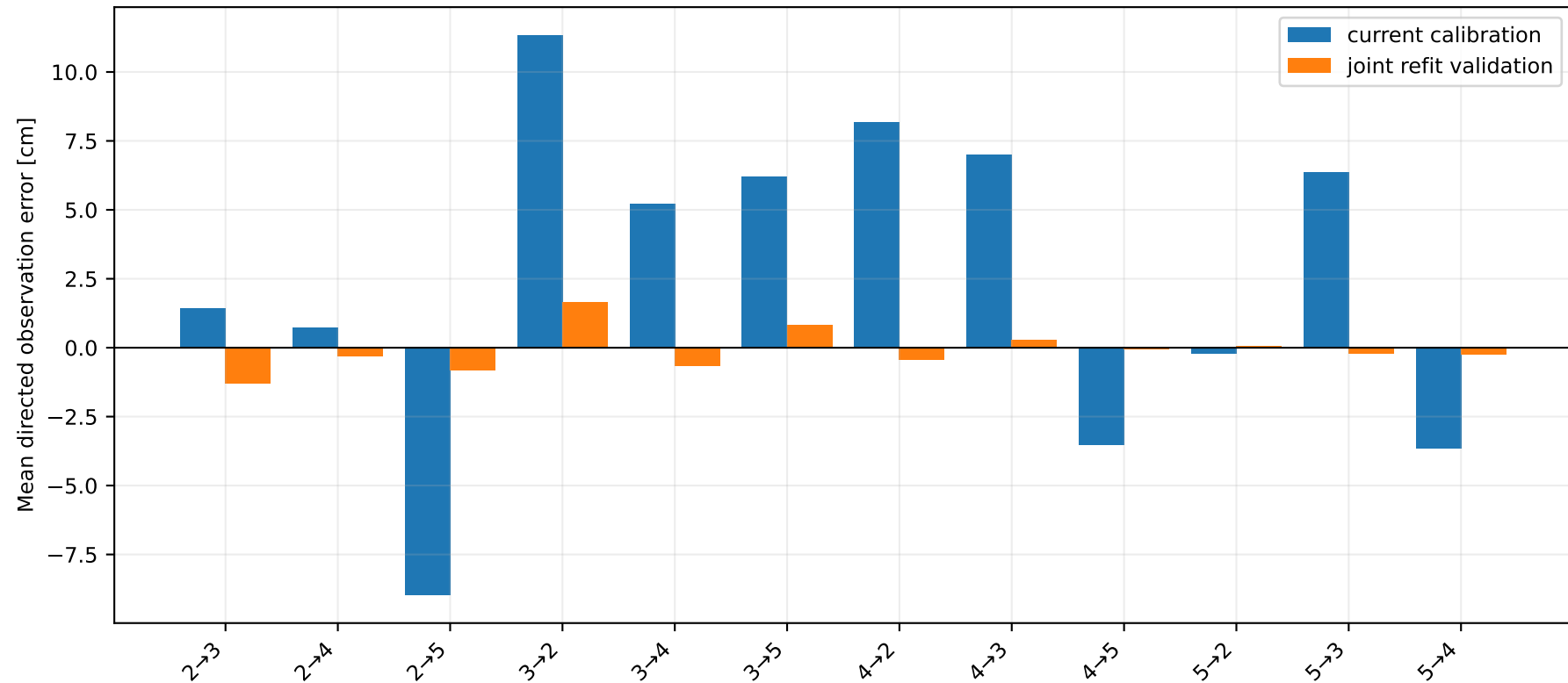
Passive DS-TWR residual bias by directed path
