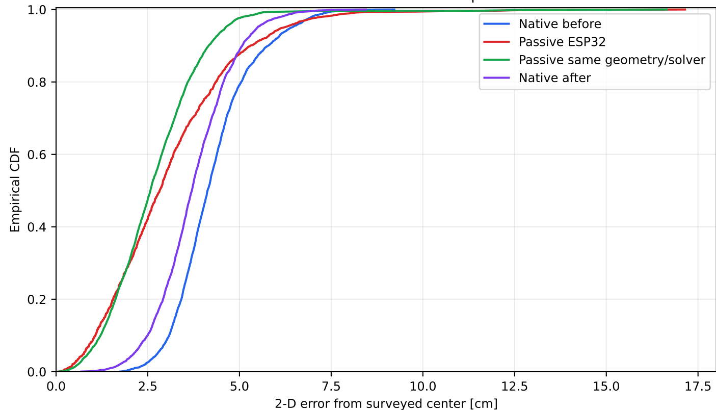
Native vs Passive DS-TWR: absolute position error
