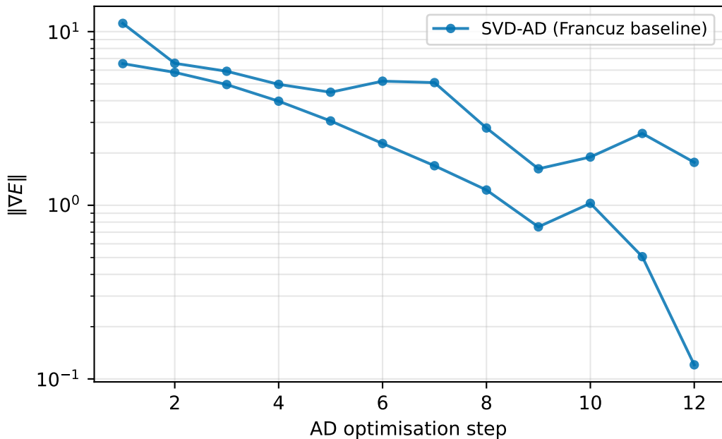
TFIM gradient norm h/J = 2.5 ( D = 2 , \chi = 8 , L-BFGS)
