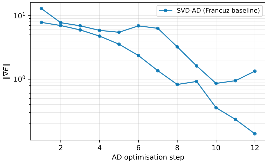
TFIM gradient norm h/J = 3.04 ( D = 2, \chi = 8 , L-BFGS)
