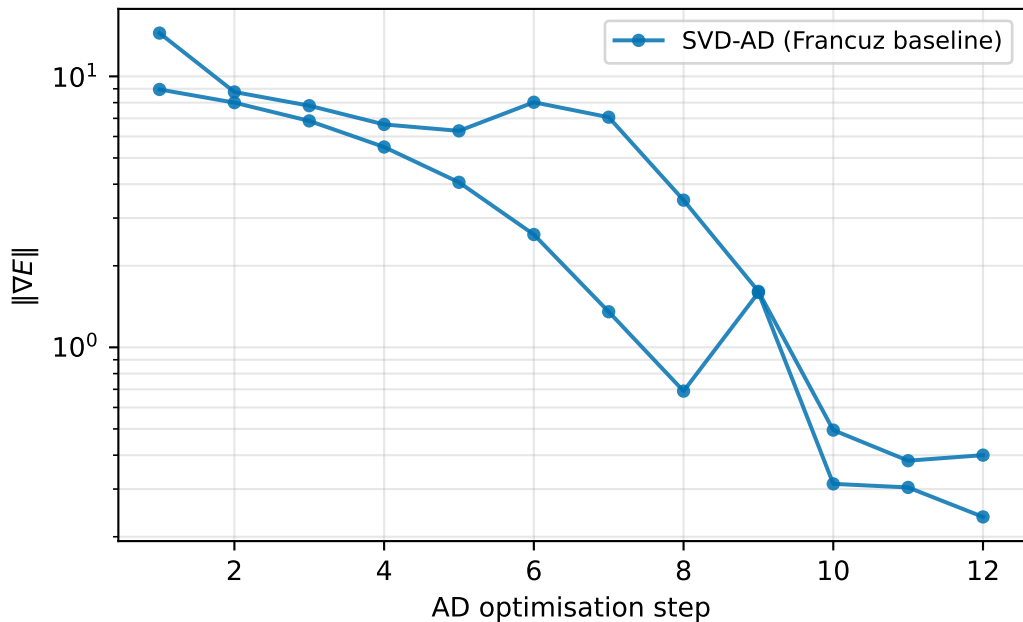
TFIM gradient norm \hbar/J = 3.5 ( D = 2 , \chi = 8 , L-BFGS)
