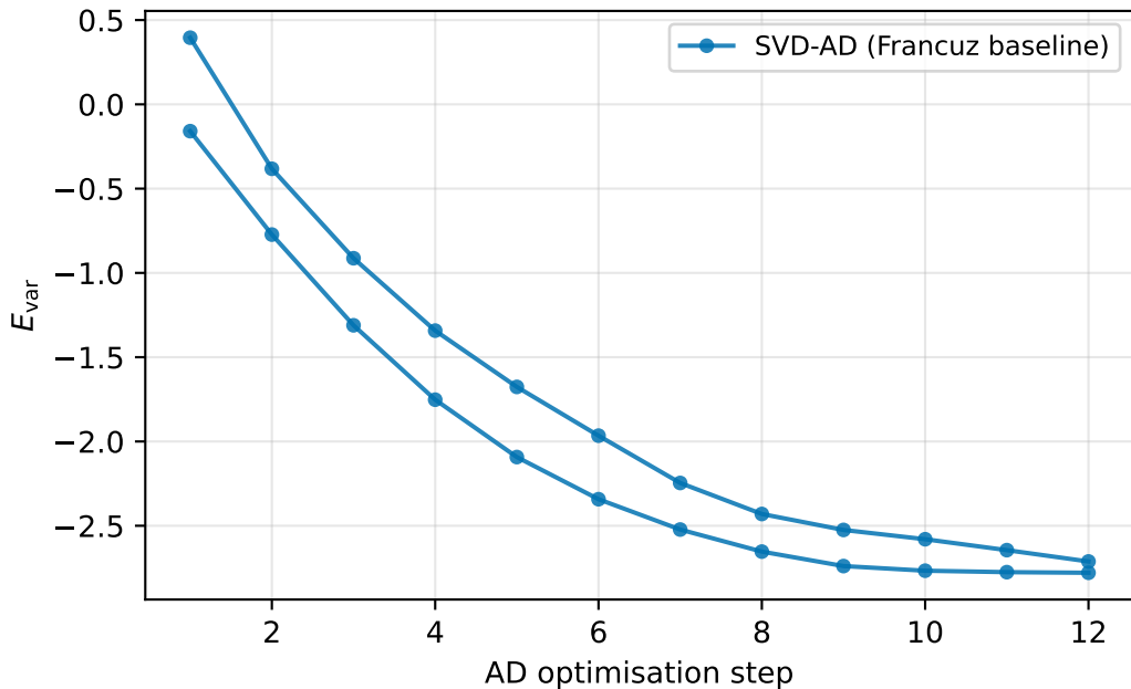
TFIM energy trajectory h/J = 2.5 ( D = 2 , \chi = 8 , L-BFGS, all seeds)
