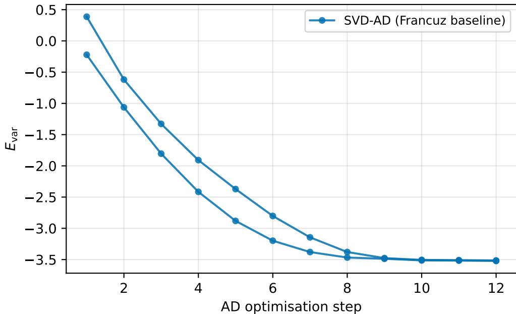
TFIM energy trajectory h/J = 3.5 ( D = 2 , \chi = 8 , L-BFGS, all seeds)
