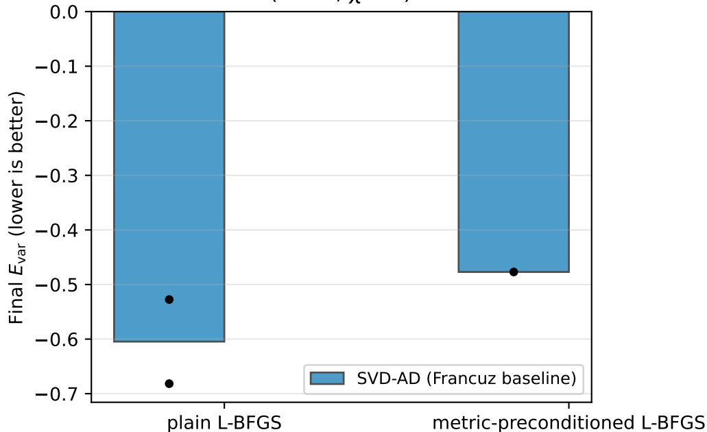
RQ5: 2 \times 2 interaction at J_1 J_2 J_2 / J_1 = 0.5 ( D = 2, \chi = 8 )
