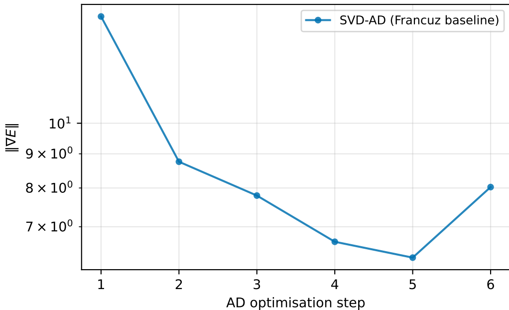
TFIM gradient norm h/J = 3.5 ( D = 2 , \chi = 8 , L-BFGS)
