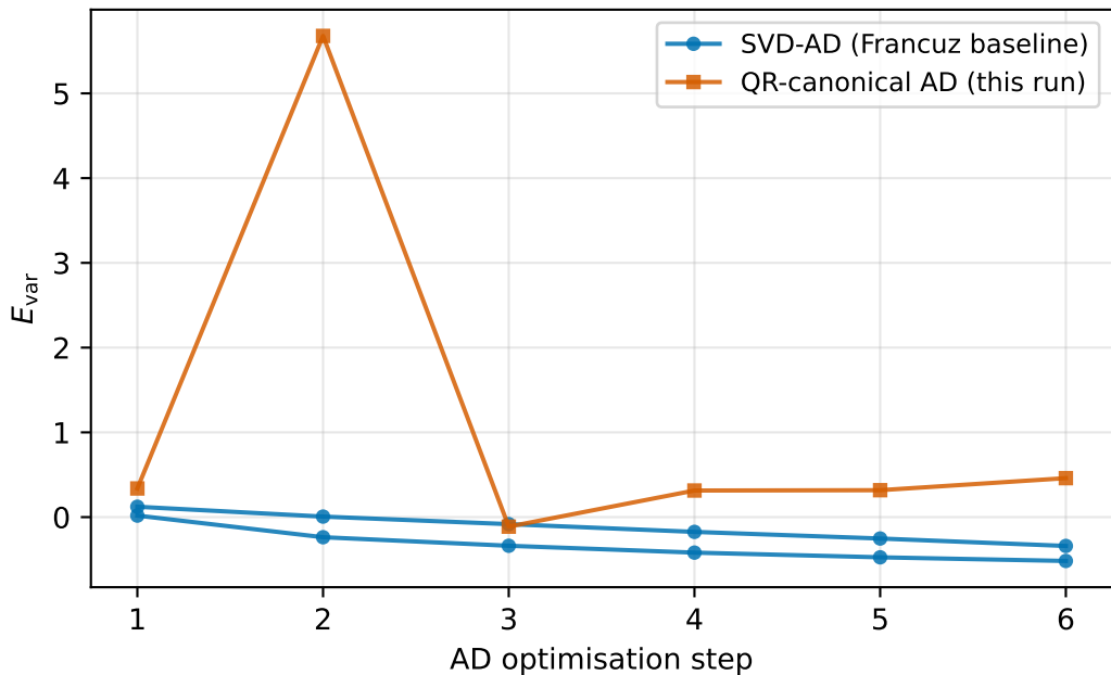
J1J2 energy trajectory J_2/J_1 = 0.0 ( D = 2 , \chi = 8 , L-BFGS, all seeds)
