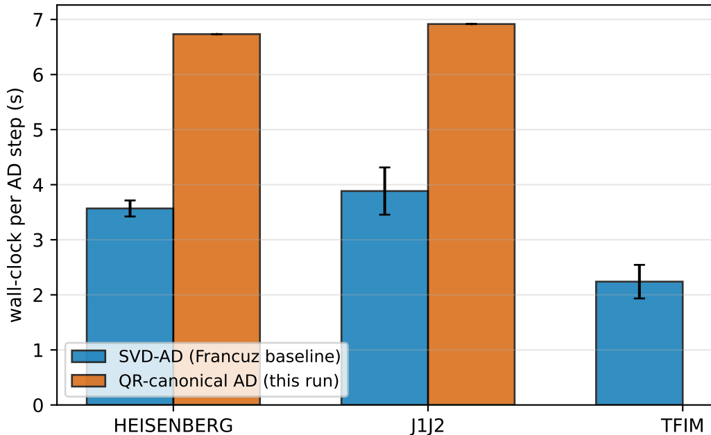
Per-step wall-clock CPU time ( D = 2 , \chi = 8 , L-BFGS, plain)
