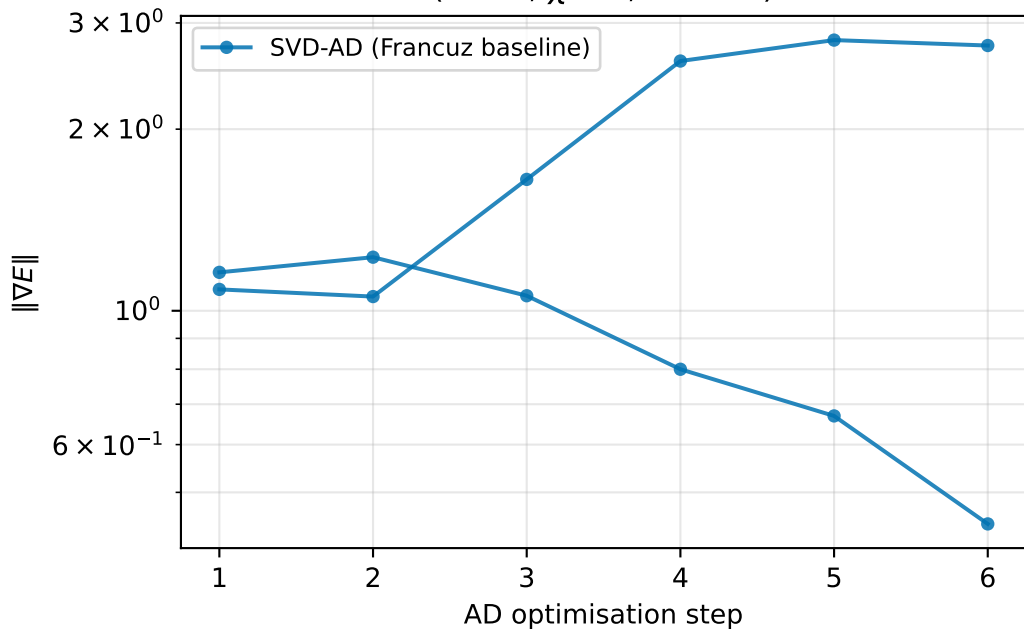
J1J2 gradient norm J_2/J_1 = 0.5 ( D = 2 , \chi = 8 , L-BFGS)
