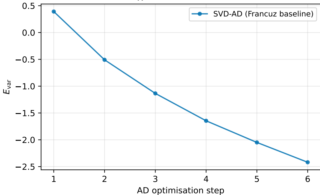
TFIM energy trajectory h/J = 3.04 ( D = 2 , \chi = 8 , L-BFGS, all seeds)
