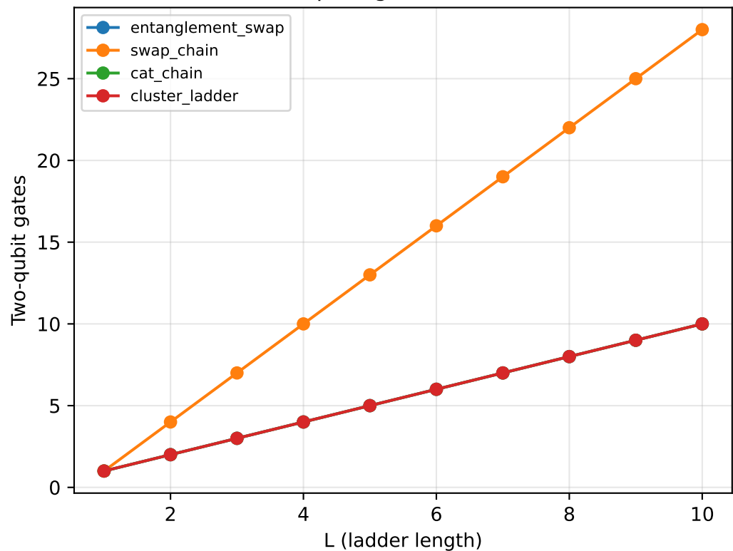
Two-qubit gate count vs L
