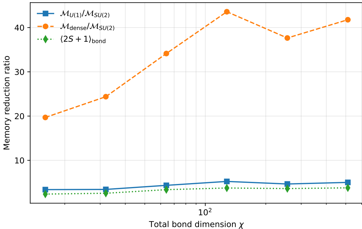
Memory reduction from abelian to non-abelian blocking
