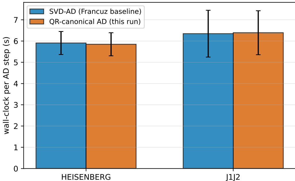
Per-step wall-clock CPU time (fixed: D = 2 , L-BFGS-plain; varying: model, ctmrg mode)
