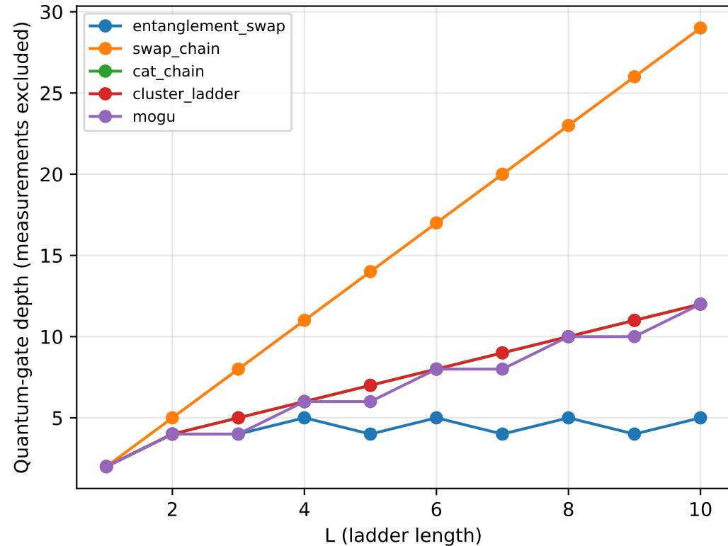
Depth vs L — quantum part only
