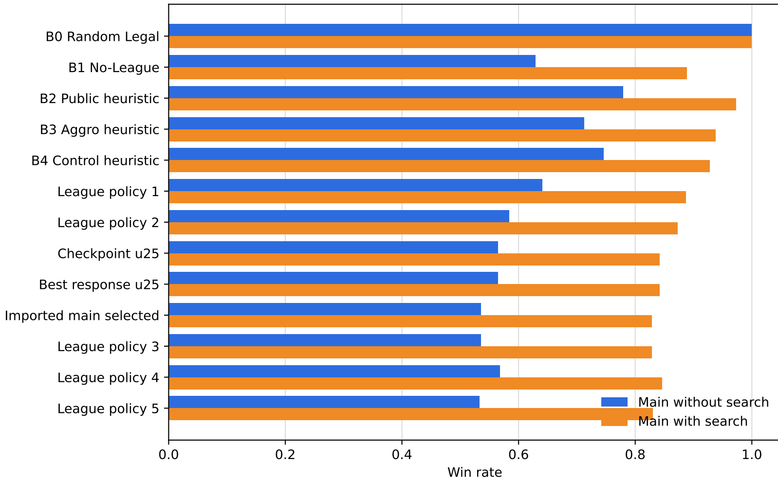
Confirm256 win rates by opponent
