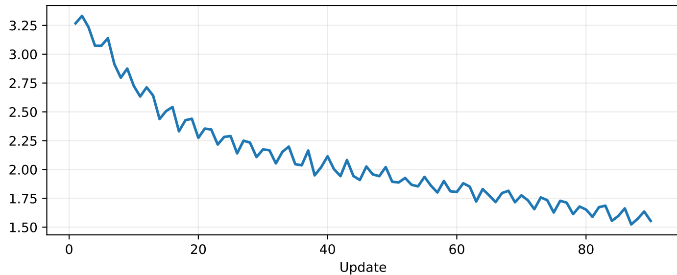
Actor loss
