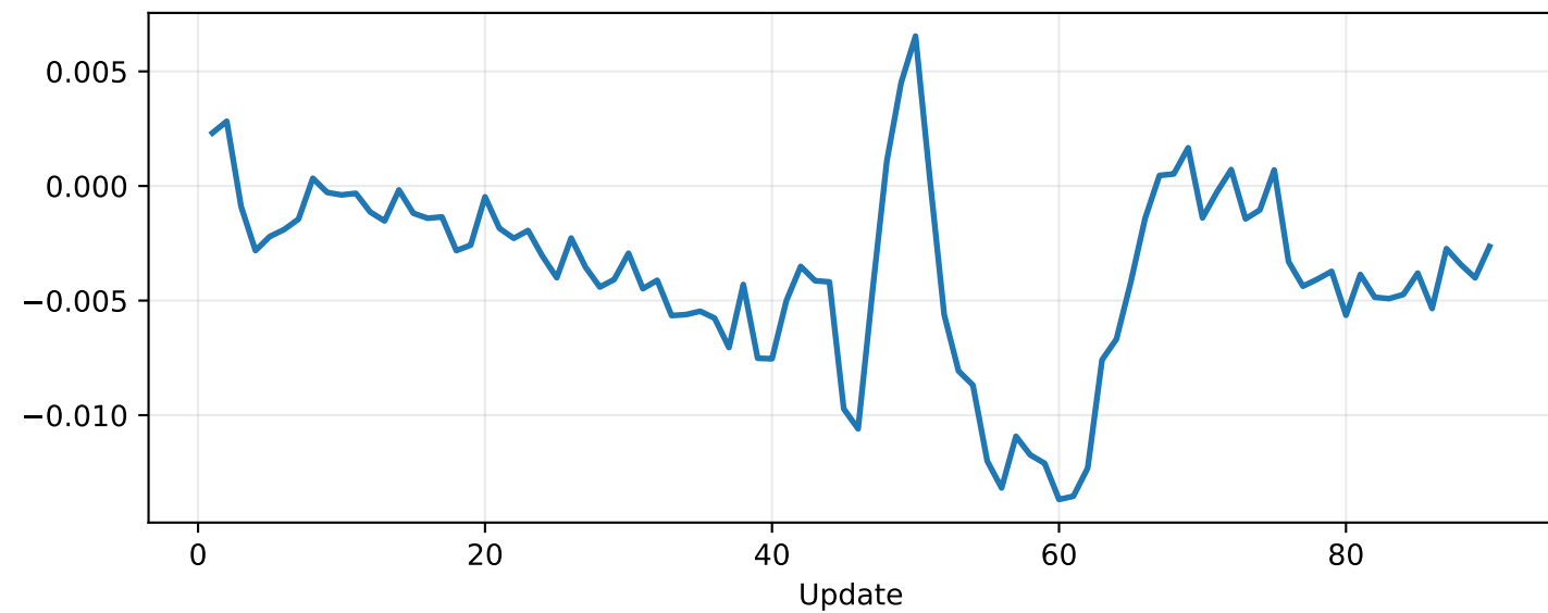
Actor loss
