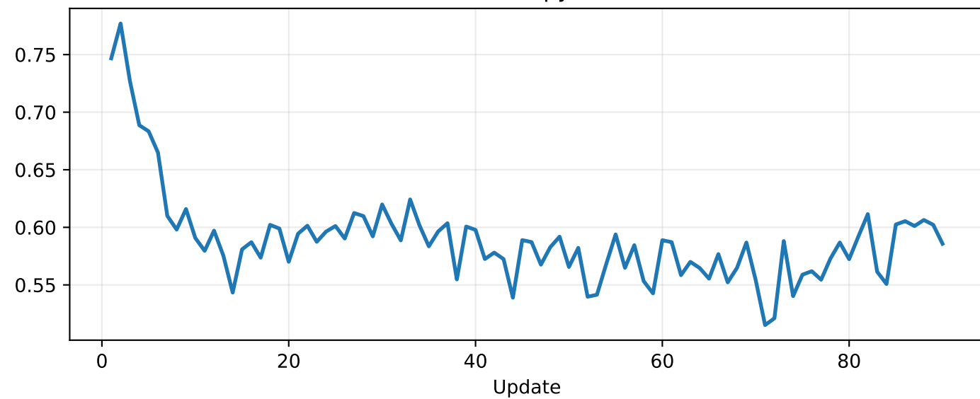
Entropy
