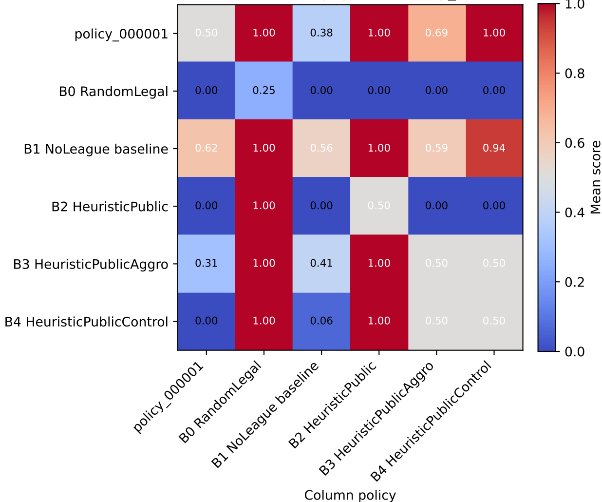
Final evaluation payoff matrix (p_mean)
