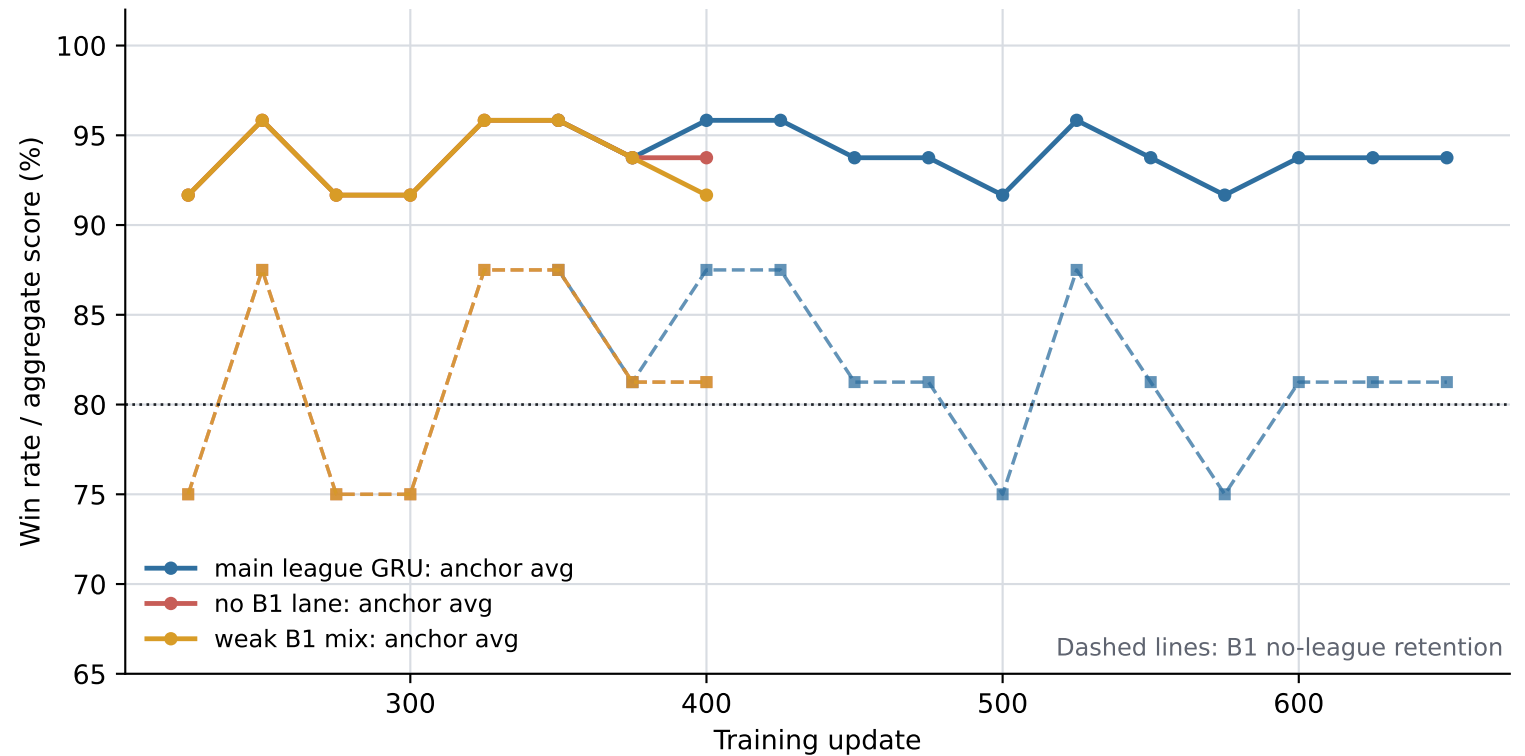
Periodic dev evaluation on fixed anchors
