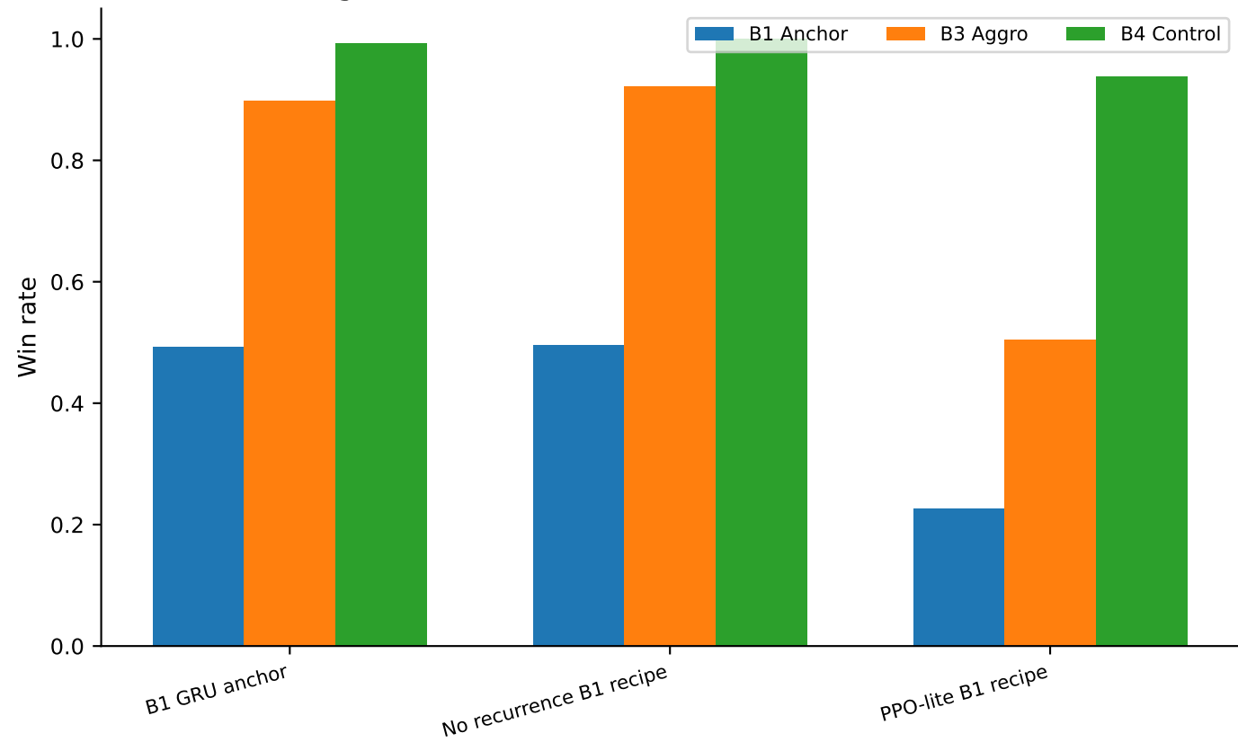
Algorithm Baseline: IMPALA/V-trace vs PPO-lite
