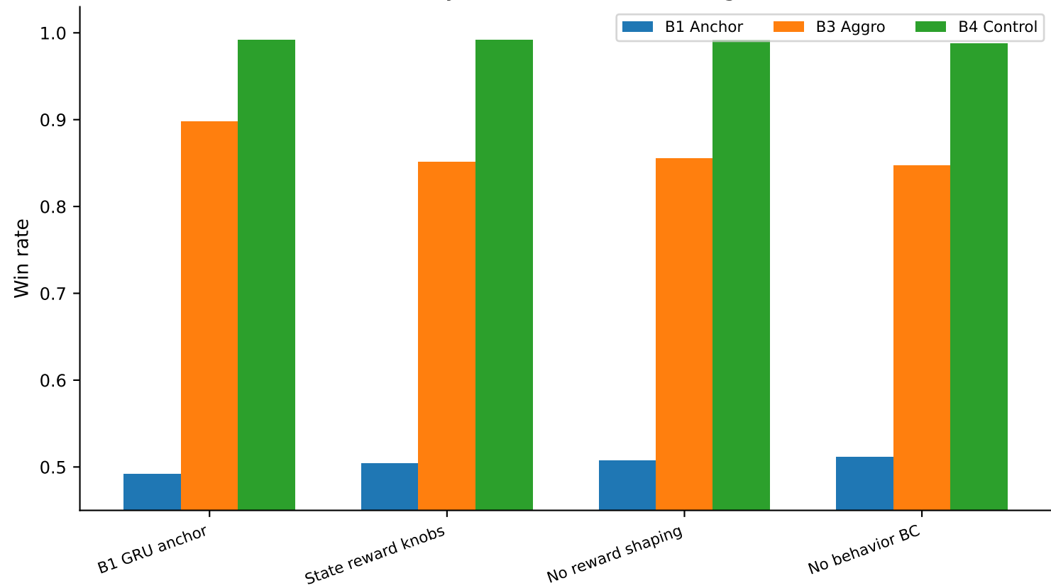
Reward/Auxiliary Ablations Trade B1 Against B3/B4
