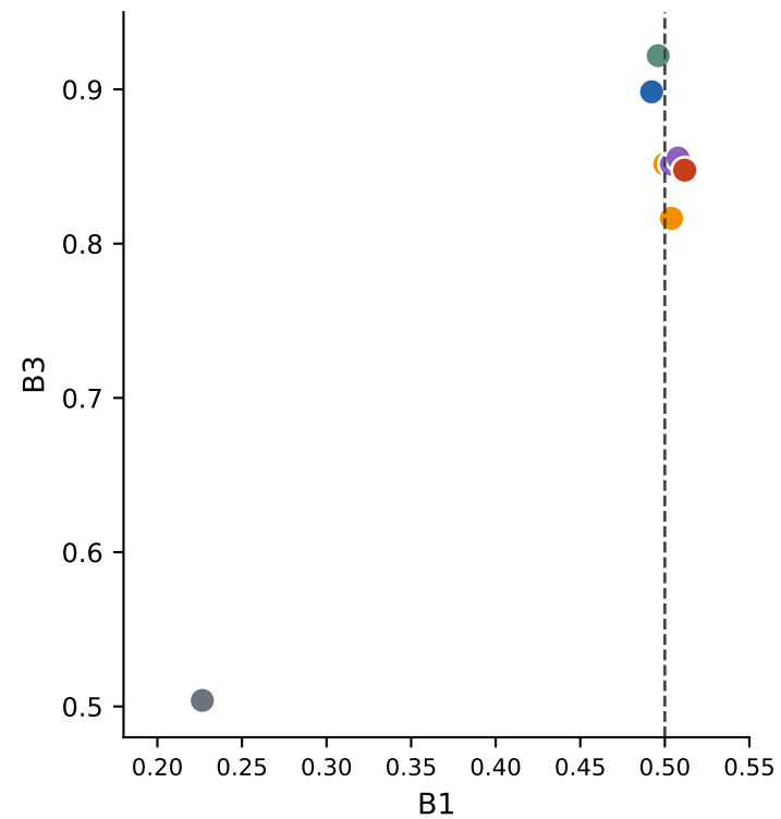
Tradeoff
