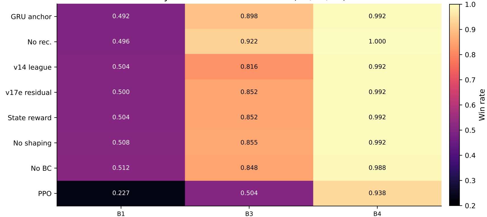
Key-Anchor Win-Rate Matrix (B1/B3/B4)
