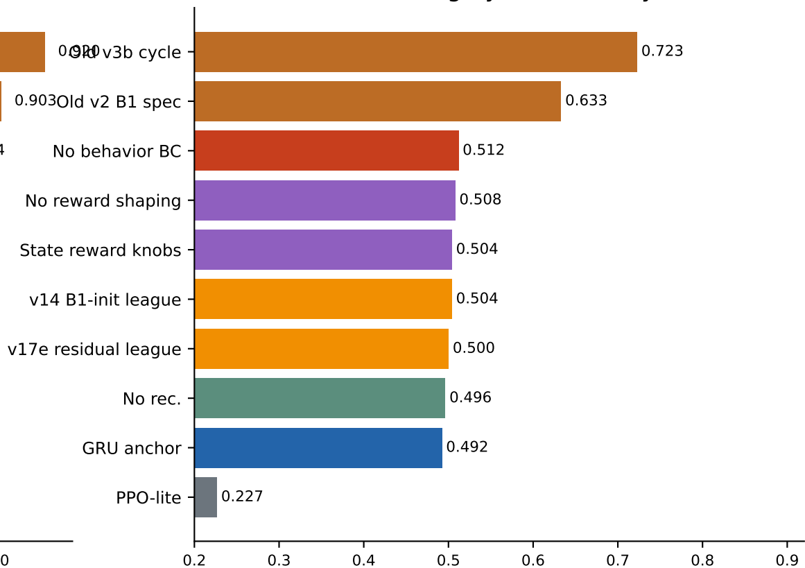
Balanced ranking by weakest key anchor
