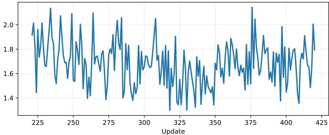
Actor loss
