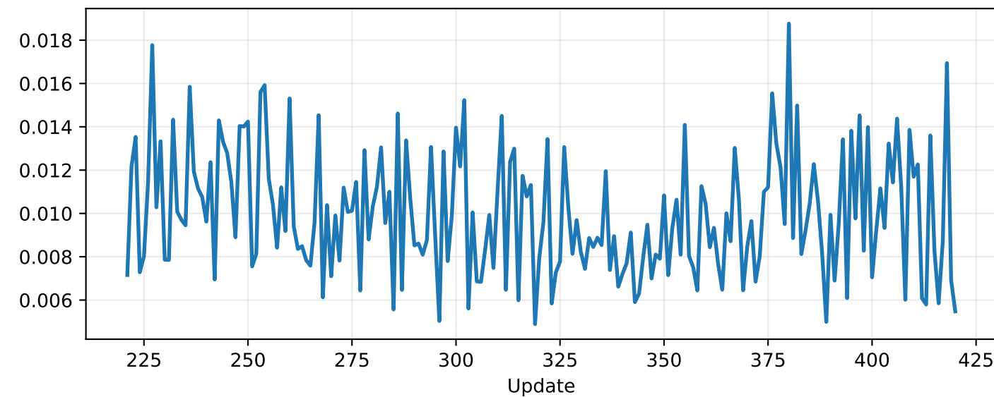
Entropy
