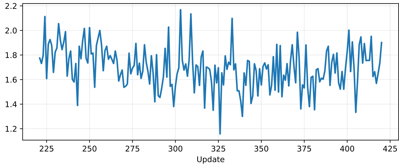
Actor loss
