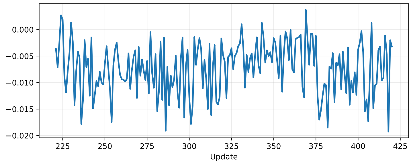
Actor loss
