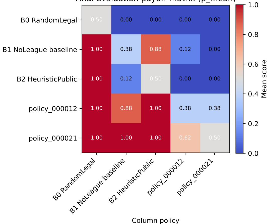
Final evaluation payoff matrix (p_mean)
