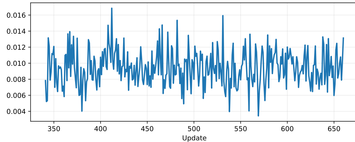
Entropy
