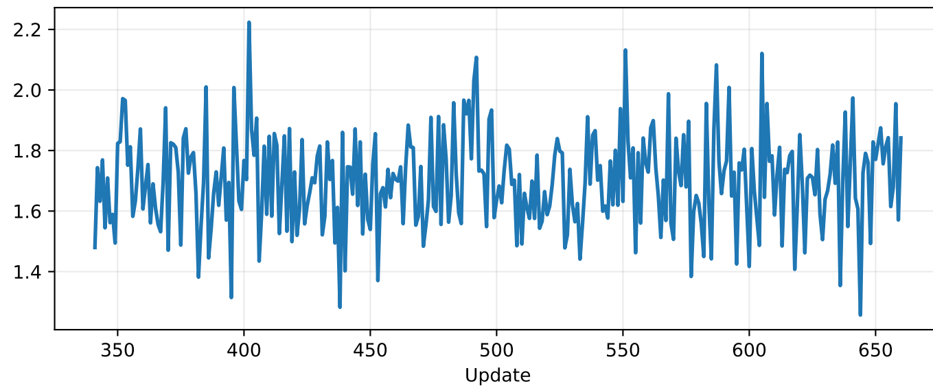
Actor loss
