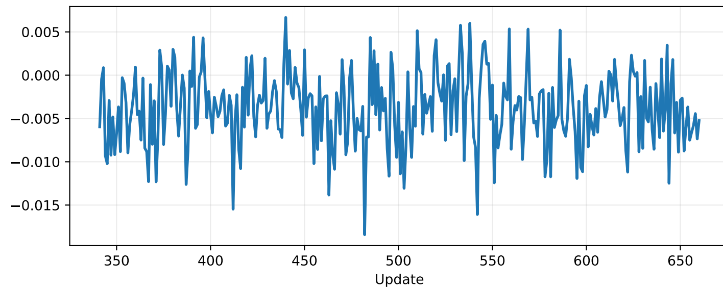
Actor loss
