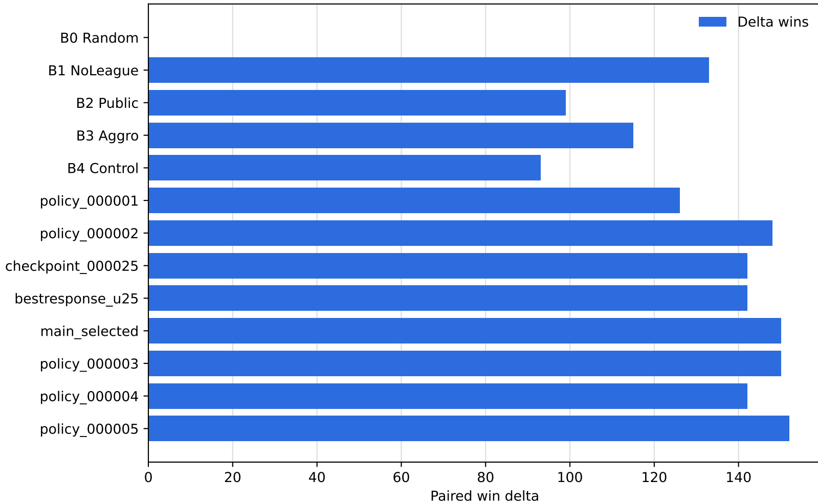
K4 search paired win deltas vs selected no-search
